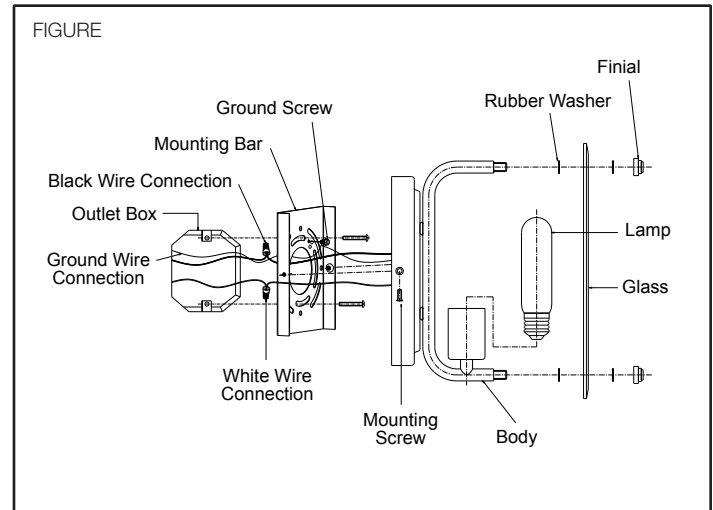
FIGURE Line art shown may not exactly match the fixture enclosed. However, the installations do apply to this fixture.
