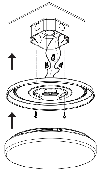
32W: 62-765, 32.5W: 62-766 Ø 19" (482.6mm) x 4.75" D (120.65mm)
