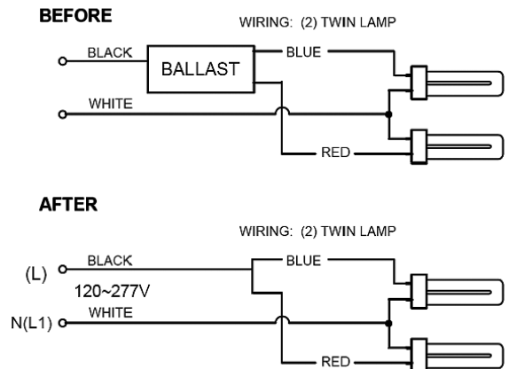
Figure 2. Retrofit with Two Lamps (GX23 & G23 base)
