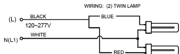
Figure 4. Retrofit with Two Lamps (GX23 & G23 base)
