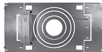
S8003 Emergency battery backup mounts directly to the 80-959 available mounting plate.
