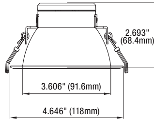
4 inch LED Commercial Downlight
