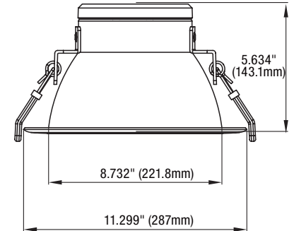
10 inch LED Commercial Downlight
