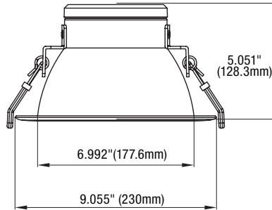
8 inch LED Commercial Downlight
