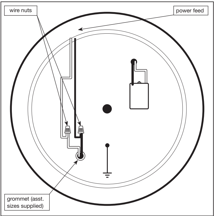
Wiring Diagram B
