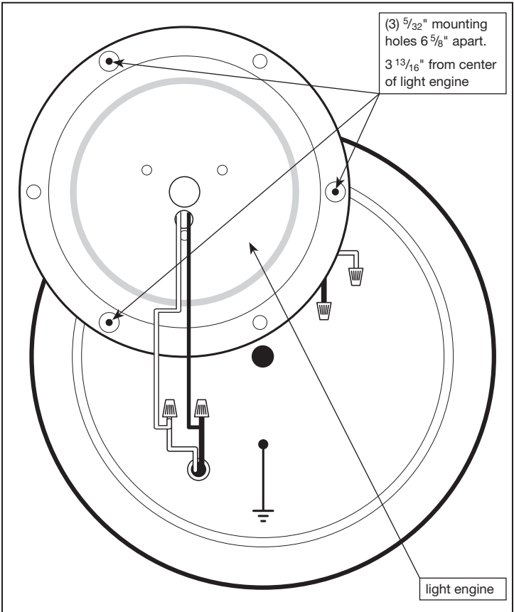
Wiring Diagram D
