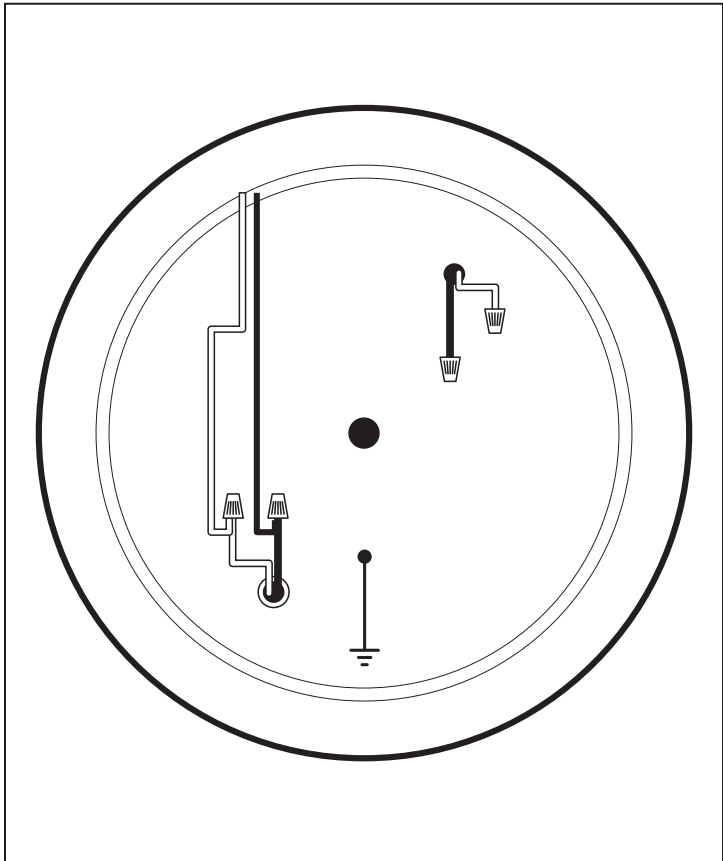
Wiring Diagram C Minimum diameter of base for use : 300mm
