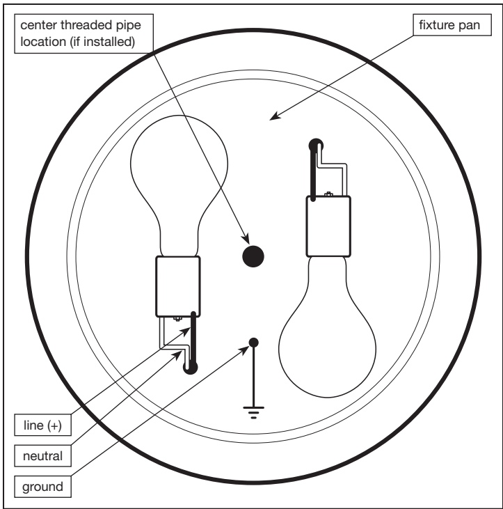
Wiring Diagram A (unaltered fixture)
