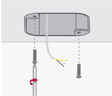
STEP 1: Turn-off /disconnect power at circuit braker.
