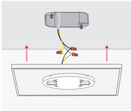
STEP 3: Make Ground connection. Attach black AC wire form fixture to black AC wire from Jbox. Connect white wire form fixture to white wire from Jbox.
