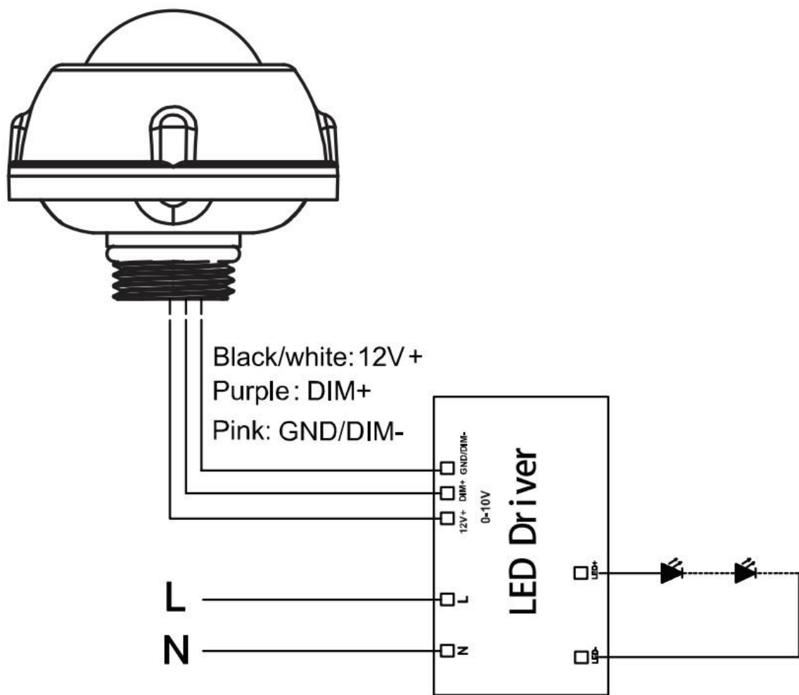
Wiring diagram
