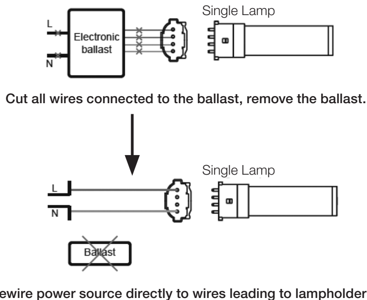
Figure 2. Electronic Ballast Wiring Modification
