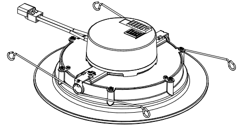
TOP ISOMETRIC
