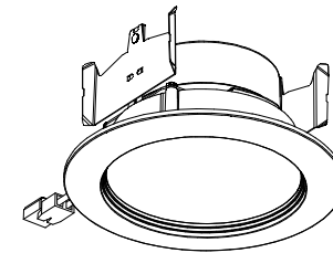
BOTTOM ISOMETRIC
