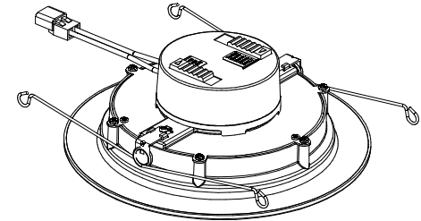
TOP ISOMETRIC
