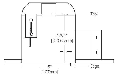
Housing
