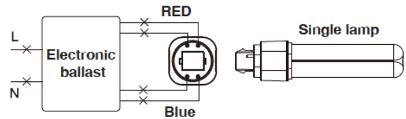
Wiring Diagram 2: Electronic Ballast
