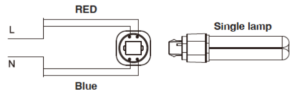
Wiring Diagram 3: Magnetic Ballast
