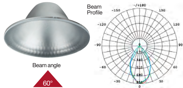
S9514 5"/6" Reflector – 60° Beam angle
