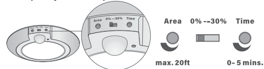
62-1313 7" & 10" with Occupancy Sensor - White Finish shown *Complies with NEC 410.16 (C)(5).
