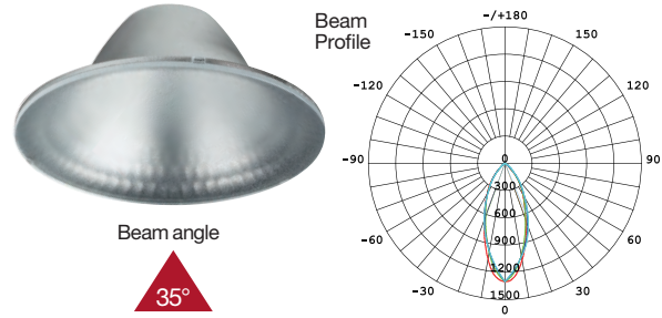
S9512 5"/6" Reflector – 35° Beam angle
