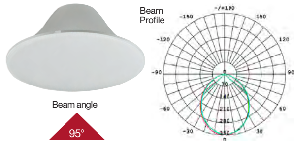
S9515 5"/6" Reflector – 95° Beam angle
