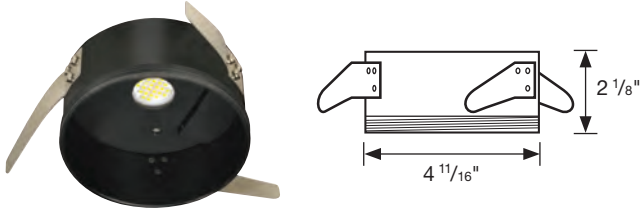
S9504 5/6" LED Housing – 13.5W, 2700K, 90CRI
