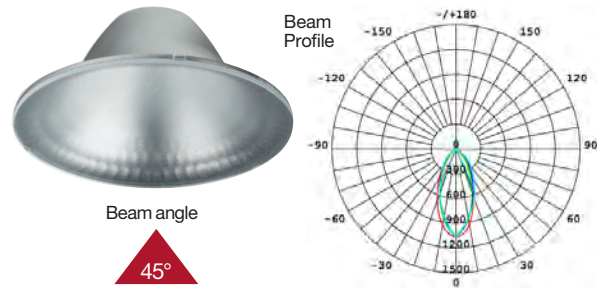
S9513 5"/6" Reflector – 45° Beam angle
