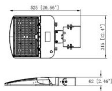
65/872 Trunnion Mount
