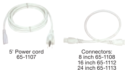
Connectible Strip Accessories
