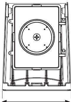
65-677, 65-678 3 7/8" (98.1±1mm) 65-679, 65-680 8 1/2" (216.1±1mm)
