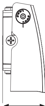
65-677, 65-678 3 7/8" (98.1±1mm) 65-679, 65-680 4 7/8" (112.1±1mm)
