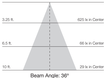
10W 36° – TH603/TH604
