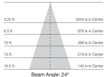
30W 24° – TH621/TH622
