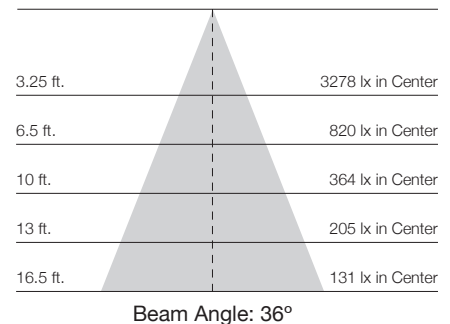
30W 36° – TH623/TH624
