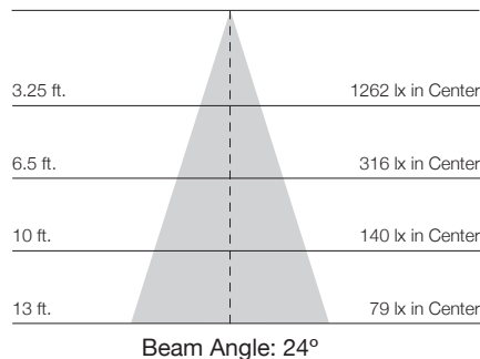
20W 24° – TH611/TH612
