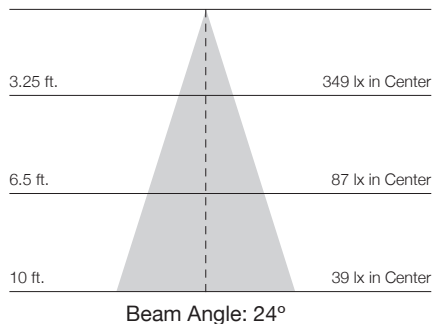
10W 24° – TH601/TH602
