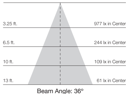
20W 36° – TH613/TH614
