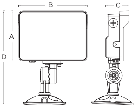
Knuckle Mount with Mounting Plate (65-542 shown)
