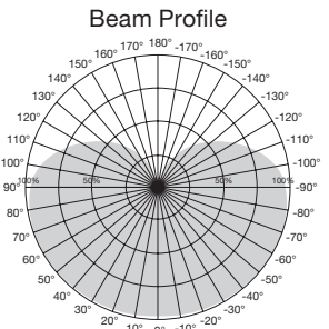
Beam Angle: 220°
