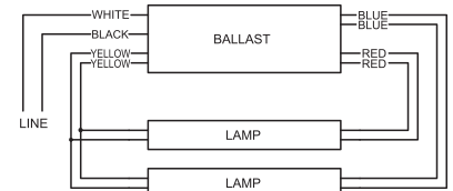
TWO LAMPS BALLAST CORRECT WIRING
