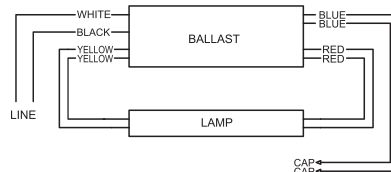
ONE LAMP BALLAST CORRECT WIRING
