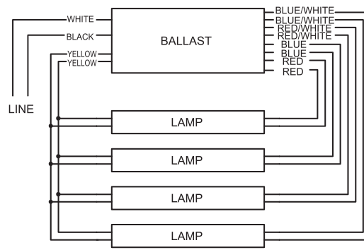
FOUR LAMPS BALLAST CORRECT WIRING
