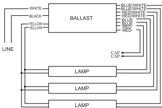
THREE LAMPS BALLAST CORRECT WIRING
