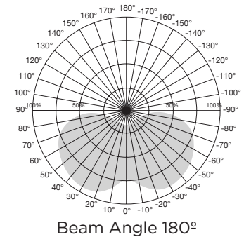
Beam Profile
