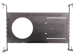
Round Rough-In Mounting Plate with Bars (80-943, 80-944)
