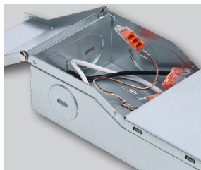
Remote Driver for Shallow Plenums
