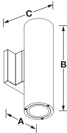
4-Inch Cylinder
